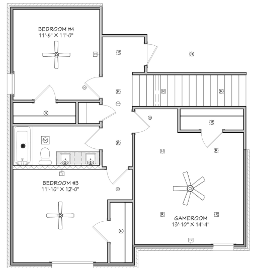
2ND FLOOR
